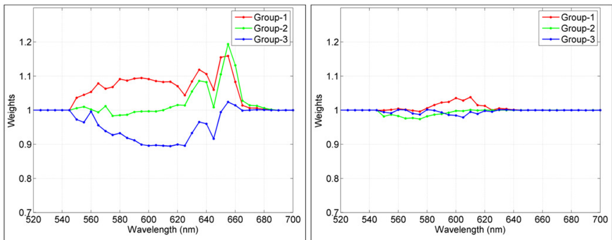
Fig. 11. (Color online) Weighting functions for the optimizing the LWS (left) and MWS (right) low density spectral absorbance. Optimization was performed above 550 nm.
