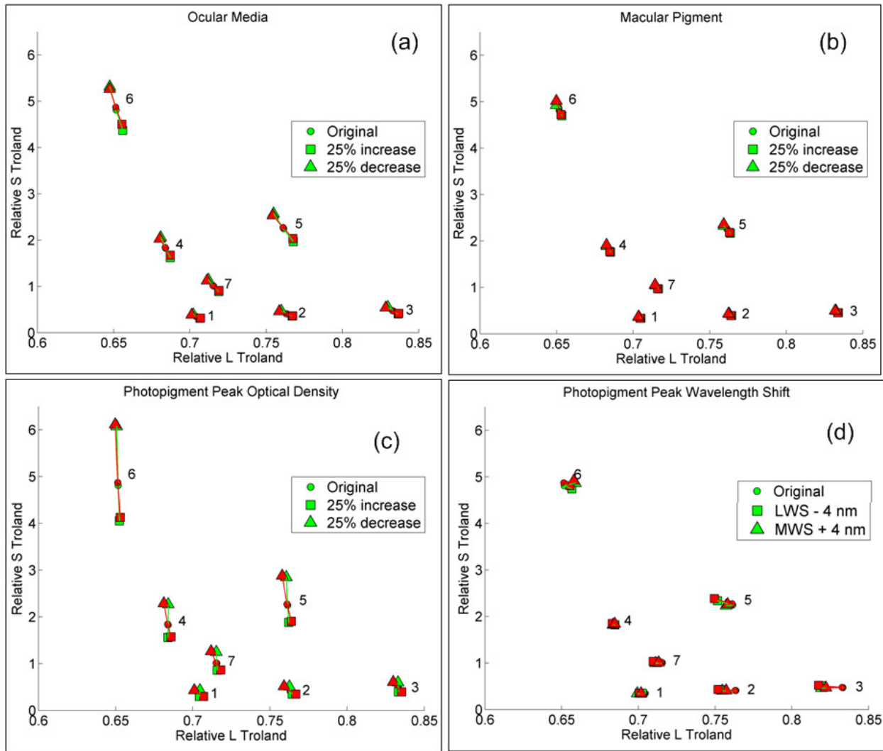
Fig. 6 (Color online) ( Note: figure should not be reduced ). Simulated chromaticity shift for seven test stimuli due to modified cone fundamentals in relative cone troland space. The circles show the original chromaticities of the stimuli. Increase (squares) and decrease (triangles) of the peak optical density by 25% are shown for ocular media (a), for macular pigment (b) and for photopigment peak optical density (c). Peak wavelength shift of LWS cone photopigment by 4 nm toward shorter wavelengths (squares) and of MWS cone photopigment by 4 nm toward longer wavelengths (triangles) are shown in (d). Green symbols correspond to the CRT and red symbols to LCD.
