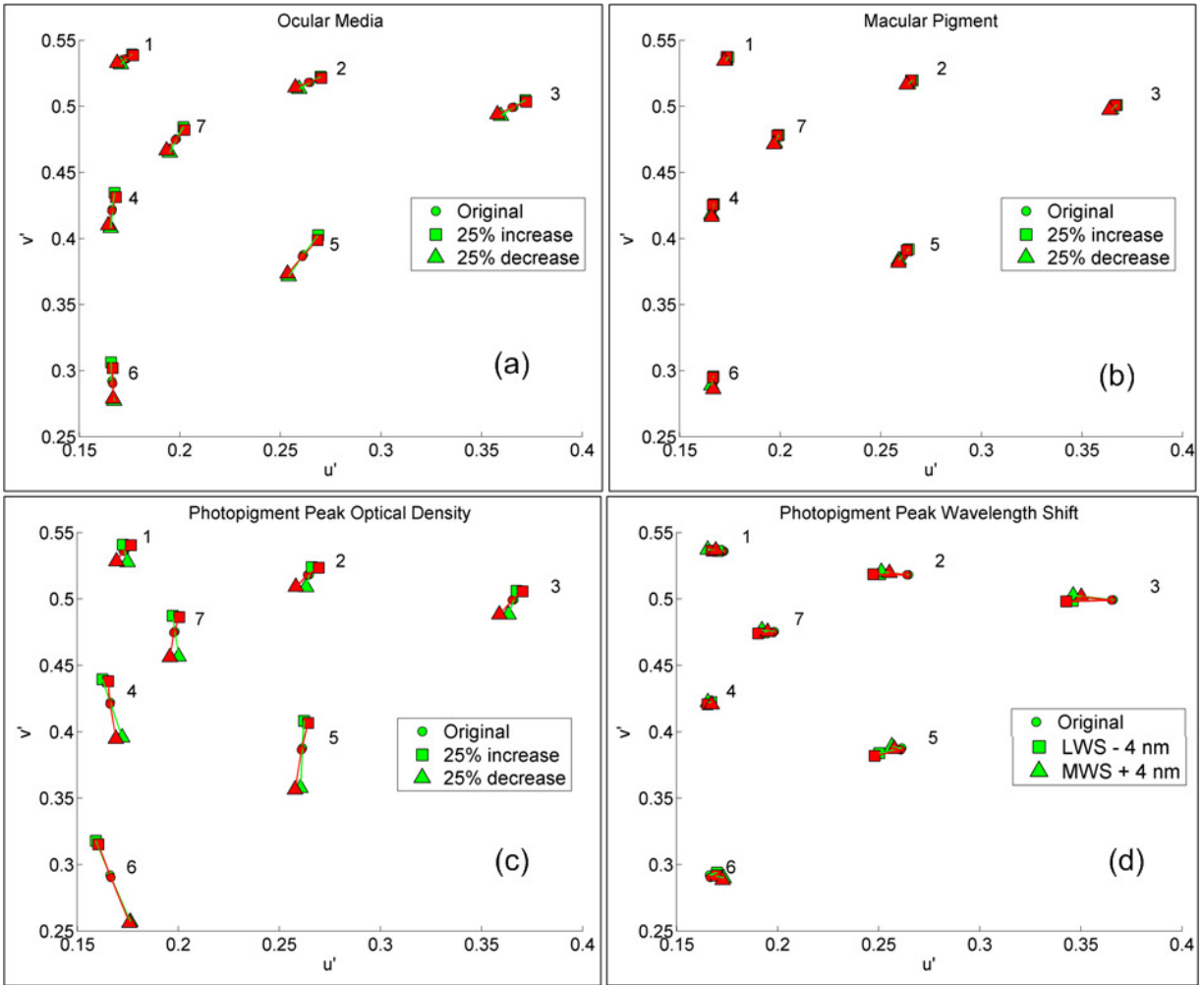
Fig. 5 (Color online) ( Note: figure should not be reduced ). Simulated chromaticity shift for seven test stimuli due to modified cone fundamentals in (u',v') chromaticity diagram. The circles show the original chromaticities of the stimuli. Increase (squares) and decrease (triangles) of the peak optical density by 25% are shown for ocular media (a), for macular pigment (b) and for photopigment peak optical density (c). Peak wavelength shift of LWS cone photopigment by 4 nm toward shorter wavelengths (squares) and of MWS cone photopigment by 4 nm toward longer wavelengths (triangles) are shown in (d). Green symbols correspond to the CRT and red symbols to LCD.
