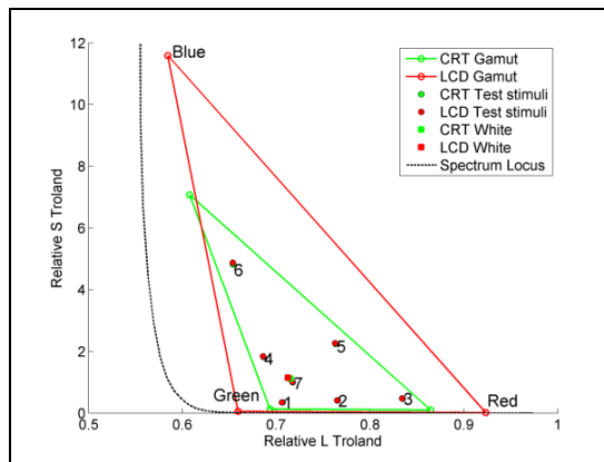
Fig. 4. (Color online) Seven test stimuli in Boynton-Kambe relative cone troland coordinates based on CIEPO6 10^\circ cone fundamentals
