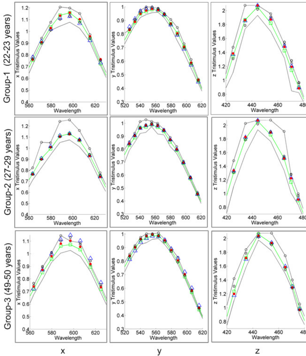
Fig. 10 (Color online) ( Note: figure should not be reduced ). CMFs for the Stiles-Burch intra-group average observer (green line with squares), CIEPO06 model predictions (blue triangles), CIEPO06 model predictions with age correspondence (red filled circles) and CIE 10° standard colorimetric observer (black star) for Group-1 (top row), -2 (middle row) and -3 (bottom row). Stiles-Burch Observers' intra-group minimum (black line) and maximum (black line with circles) are also shown. Each plot shows the CMFs around the peak only.
