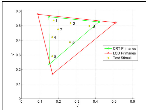
Fig. 3. (Color online) Seven test stimuli in (u', v') chromaticity diagram
