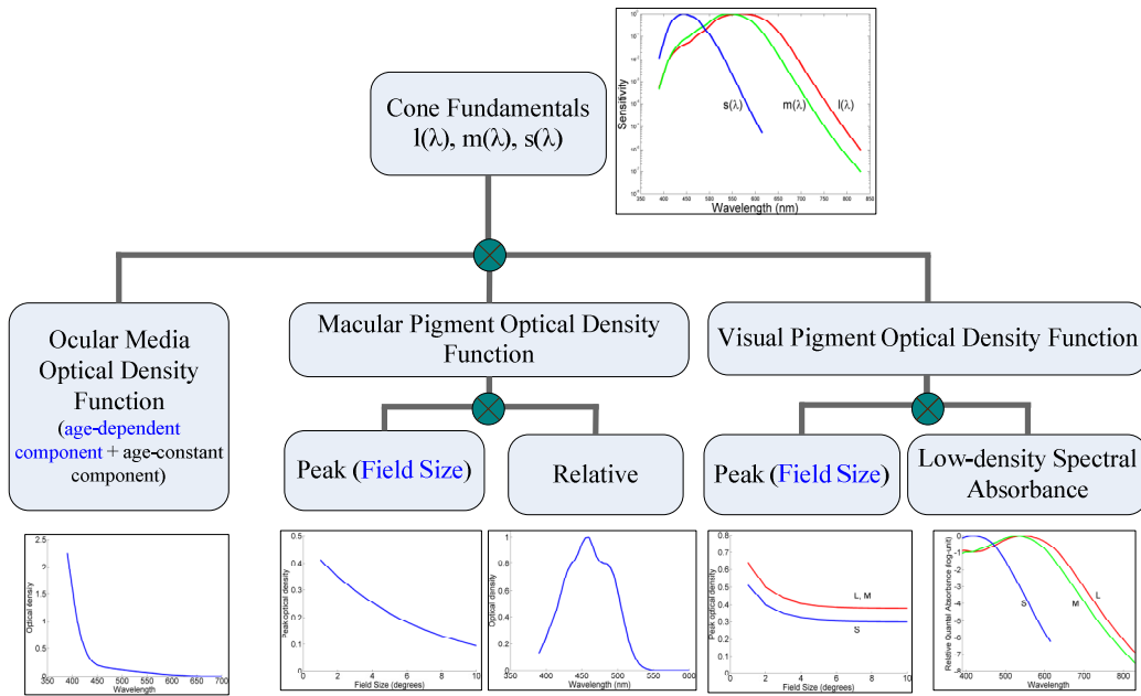
Fig. 1. (Color online) A block diagram of the CIEPO06 framework
